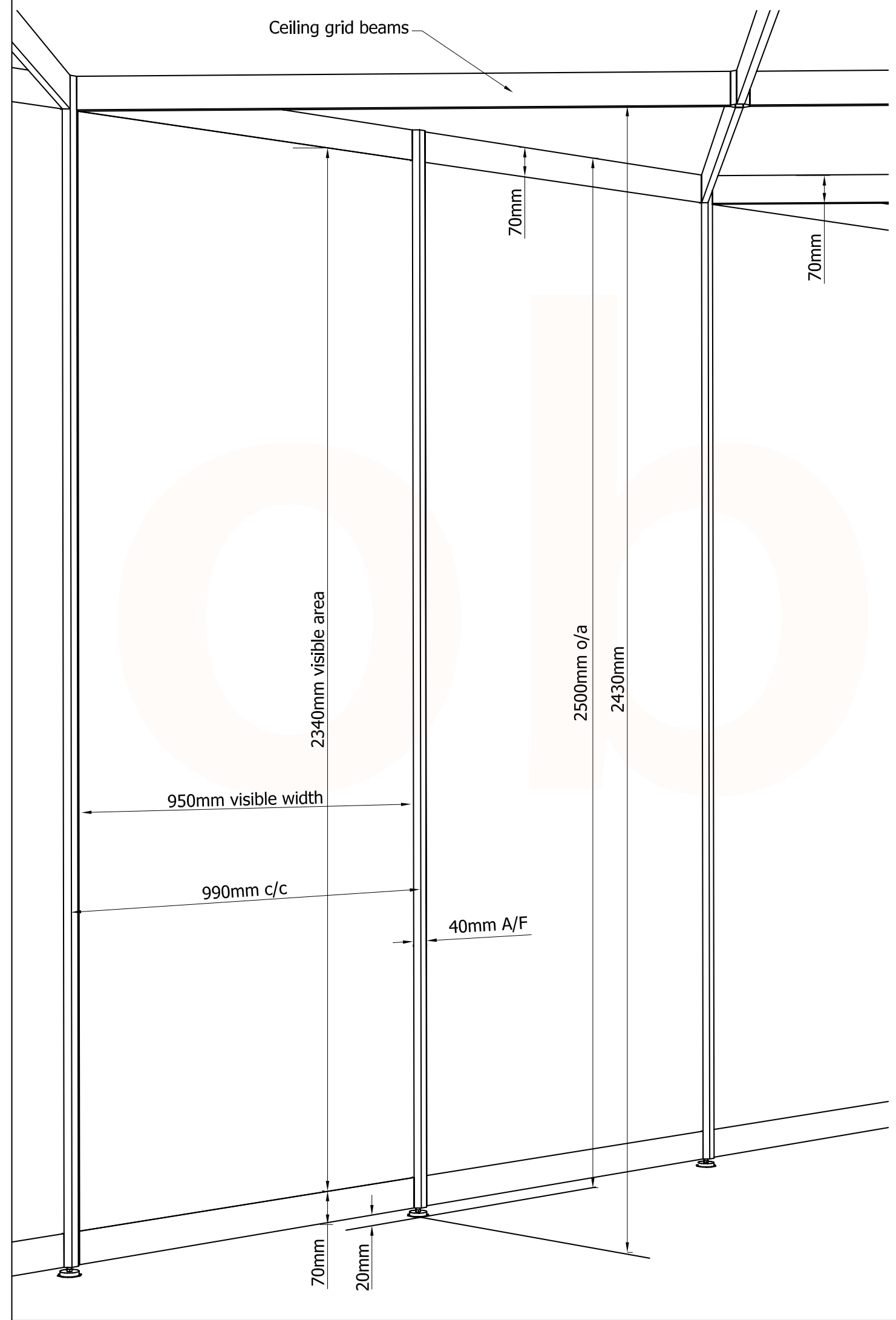
Shell Scheme typical internal appearance and dimensions.
